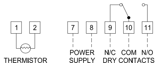
Figure 2: DLC Wiring
